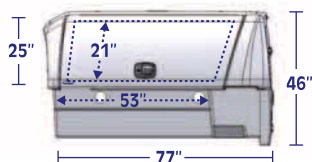
M-90 6' bed - Weight with access doors: 360 lbs / without: 315 lbs - Internal volume: 90 c.f
