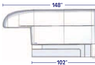
V-365 8' bed Weight: 700 lbs - Internal volume: 365 c.f
