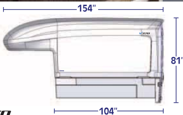
V-370 8' bed - Weight: 860 lbs - Internal volume: 370 c.f
